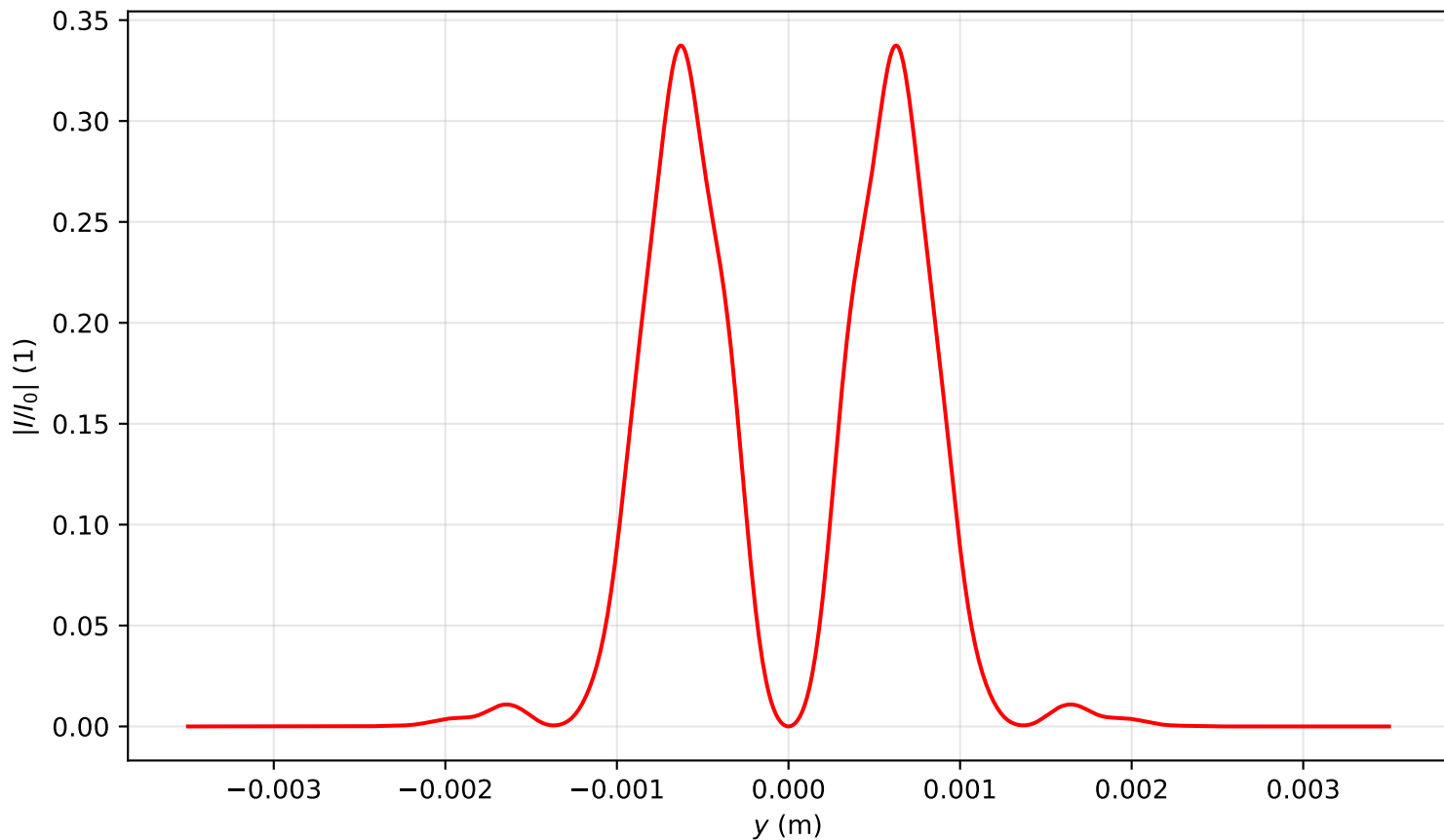
Intensity profile I(x=0, y, z=1.672)/I_0 , \text{Pin}=5.0\text{Pcr} , artificial time
